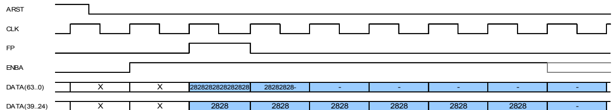
Figure 2 SONET / SDH Frame Alignment
