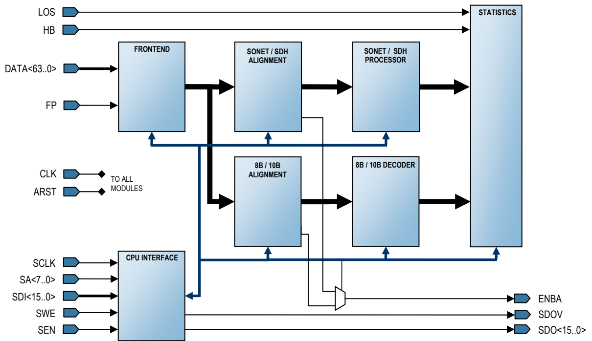
Figure 1 Block Diagram
